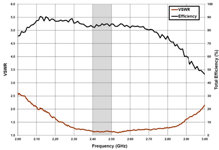
Figure 9: 2400 MHz efficiency figures
