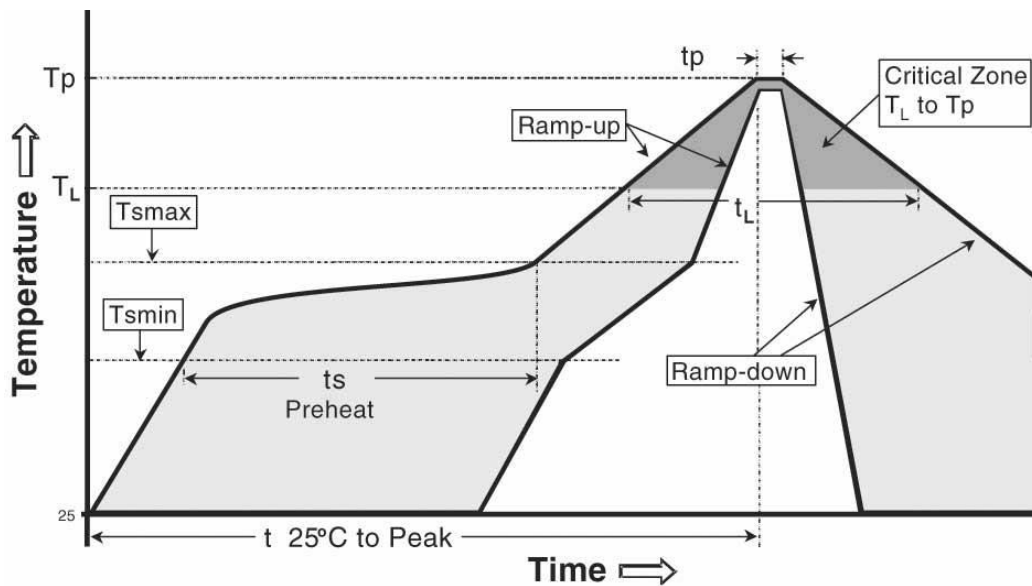
Figure 15: temperature profile for soldering
