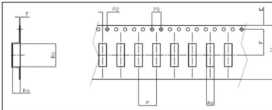
Figure 16: tape dimensions and tolerances
