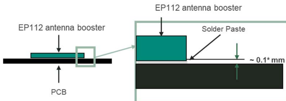
Figure 14: soldering details
