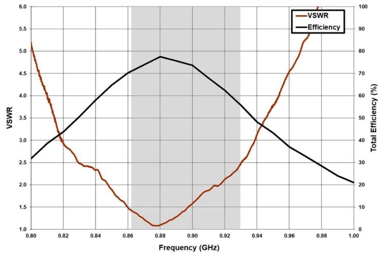
Figure 6: 900 MHz efficiency figures
