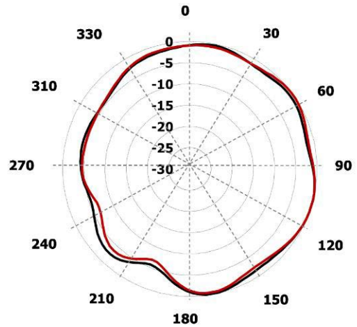
\phi = 90^\circ Plane YZ at 868 MHz & 915 MHz
