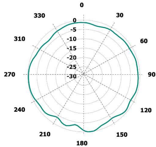
\phi = 90^\circ Plane YZ at 2450 MHz
