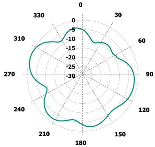
\theta = 90^\circ plane XY at 2450 MHz
