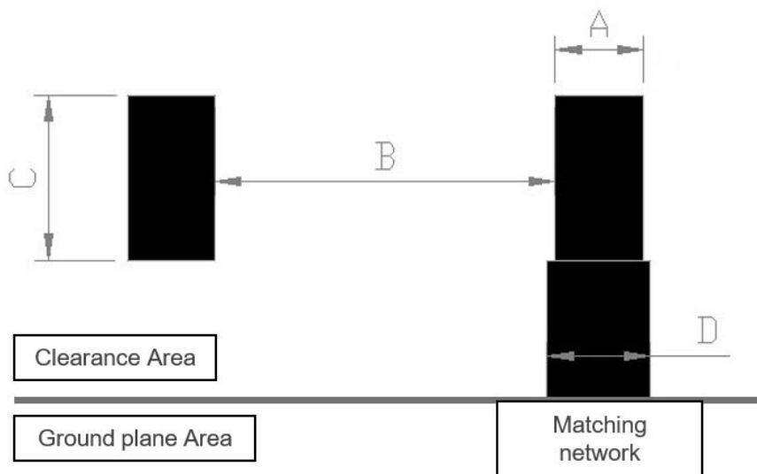
Figure 12: Footprint dimension for a single instance
