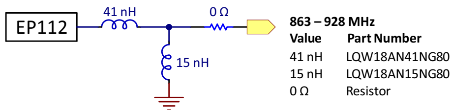
Figure 2: matching network example for 869-928 MHz frequency range (as on 900 MHz EVK)
