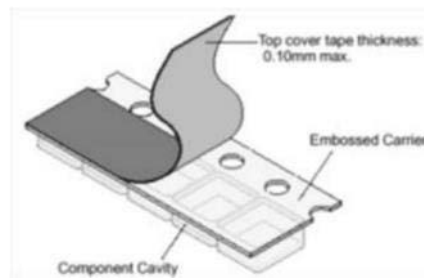
Figure 17: image of the tape
