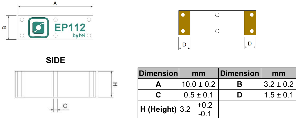
Figure 11: mechanical drawing
