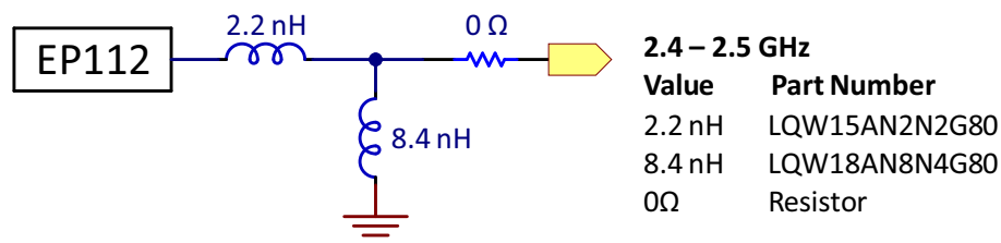
Figure 3: matching network example for 2.4-2.5 GHz frequency range (as on 2540 MHz EVK)
