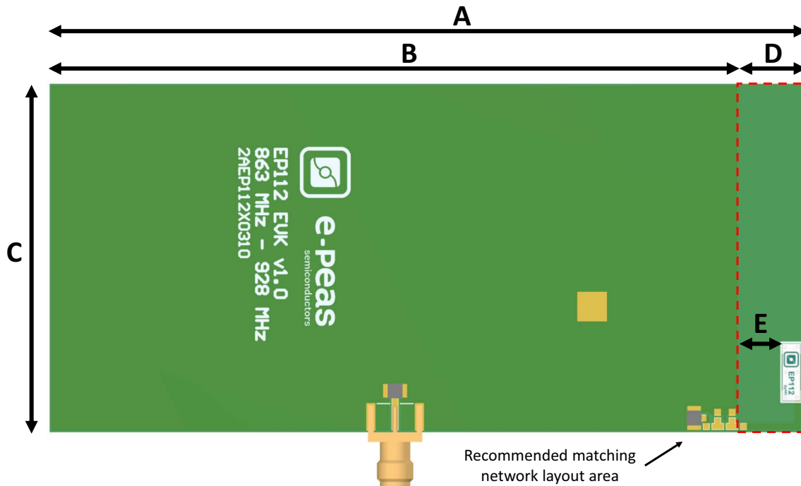
Figure 5: EP112 863-928 MHz EVK dimensions (drawing)
