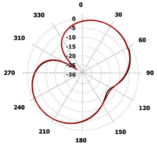
\theta = 90^\circ plane XY at 868 MHz & 915 MHz
