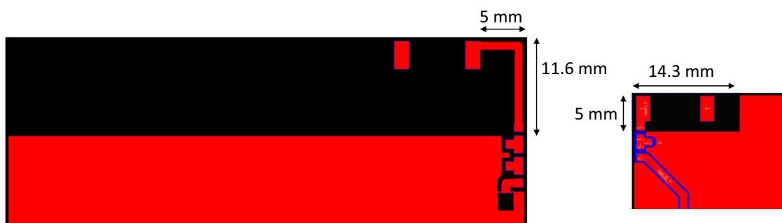
Figure 4: PCB tracks routing examples (left: 900MHz; right: 2.45GHz)
