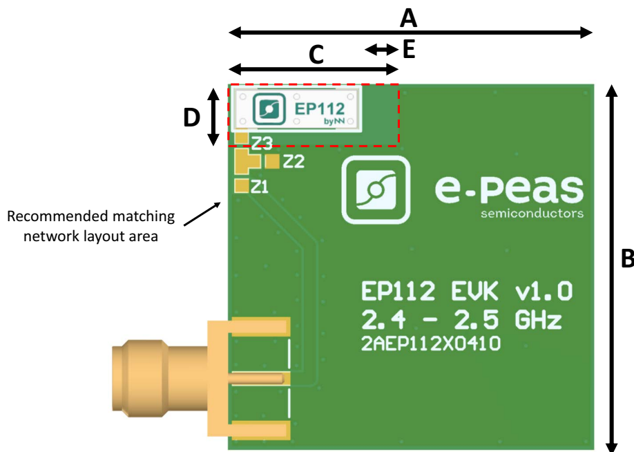
Figure 8: EP112 2.4-2.5 GHz EVK dimensions (drawing)
