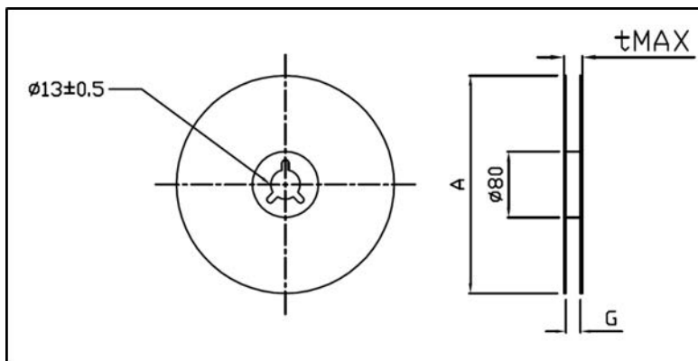
Figure 18: reel details
