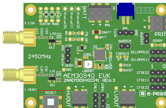
Figure 2: Board Reset
