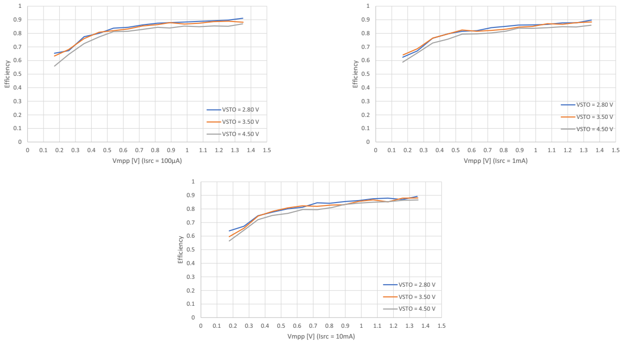
Figure 2: DCDC Conversion Efficiency
