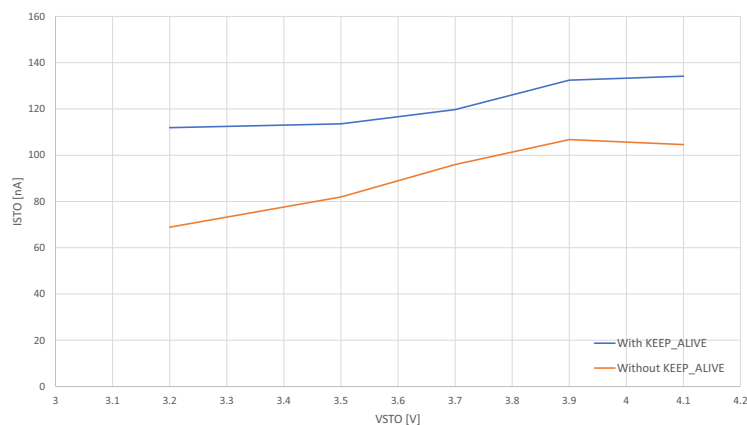
Figure 3: Quiescent Current
