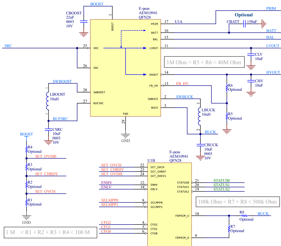
Figure 24: Schematic example
