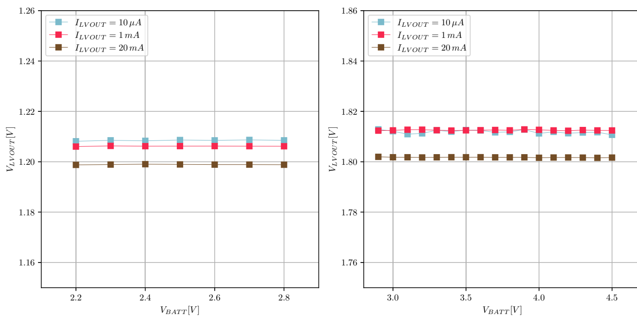
Figure 21: LVOUT at 1.2 V and 1.8 V
