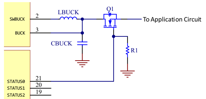
Figure 8: Schematic for supplying an application circuit with BUCK
