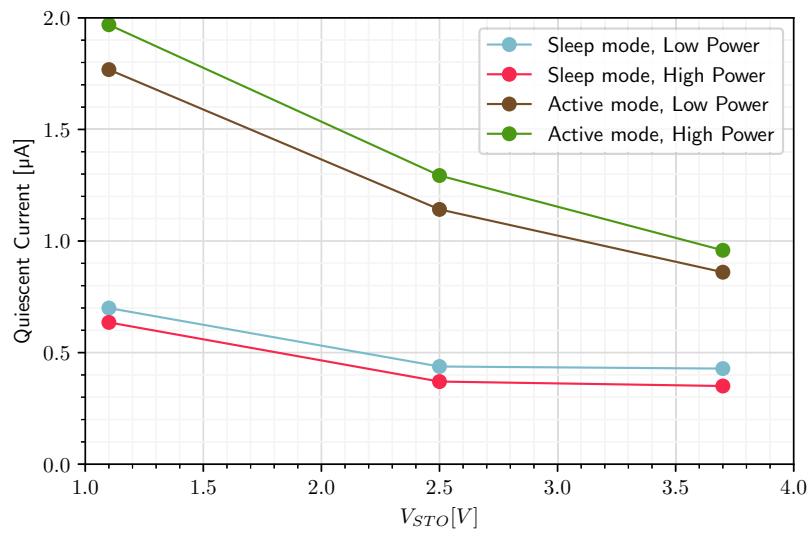
Figure 16: Quiescent Current
