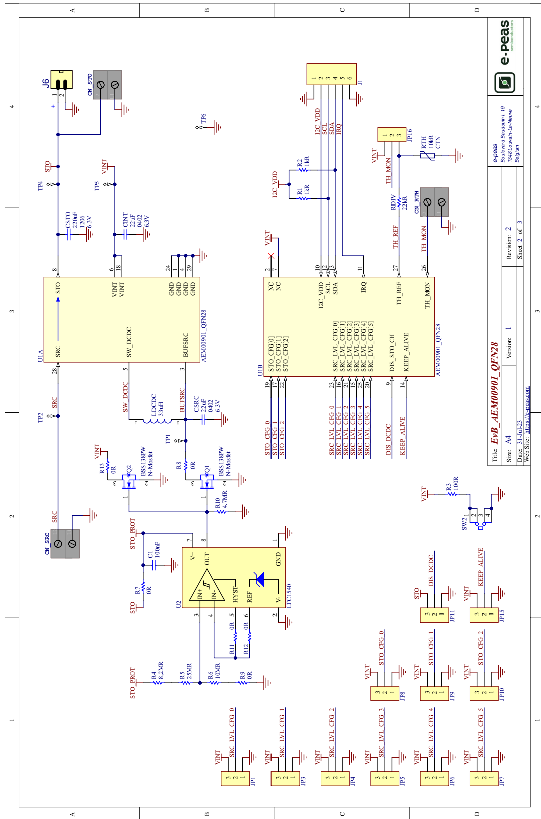
Figure 3: AEM00901 Evaluation Board Schematic
