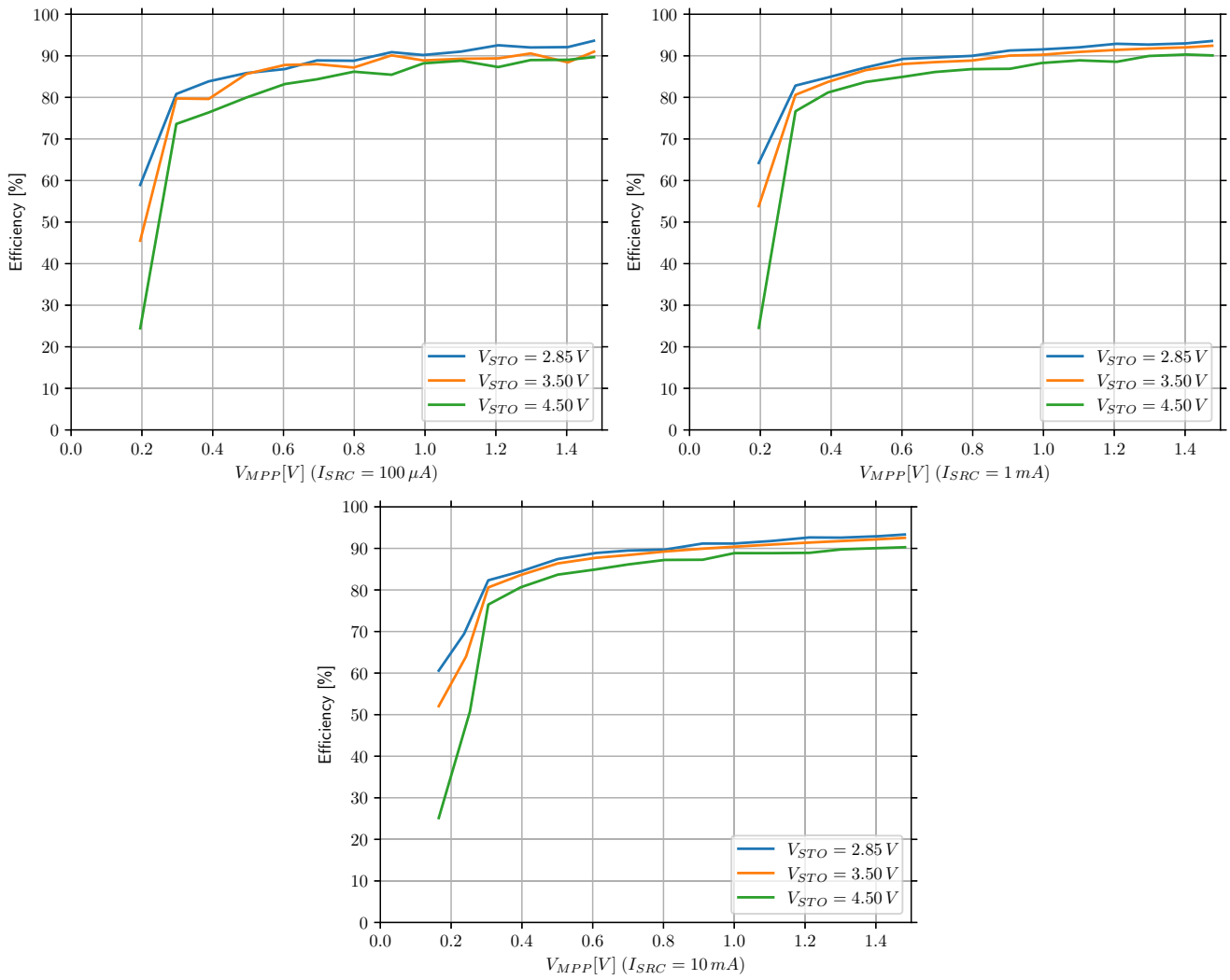
Figure 2: AEM00901 efficiency (LDCDC: Coilcraft LPS4018-333MRB)
